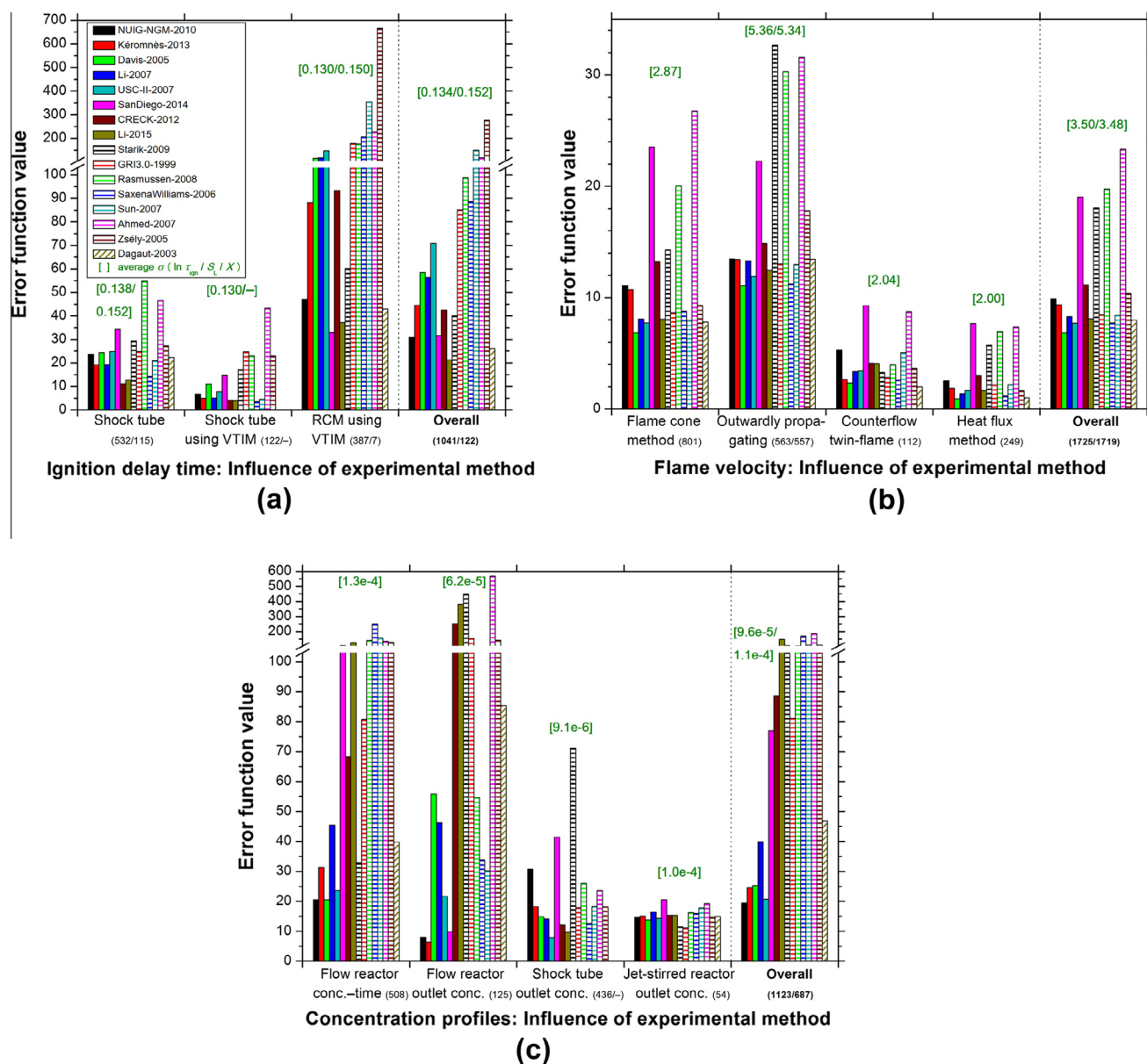
Fig. 1. Errors of the reproduction of (a) ignition delay times, (b) flame velocities and (c) concentration profiles according to the respective type of experiment. The numbers in parentheses indicate the number of data points included. The 2 nd values refer to the number of data points for Dagaut-2003. Green numbers above the columns refer to average \sigma values for each subset. All diluents except He.
