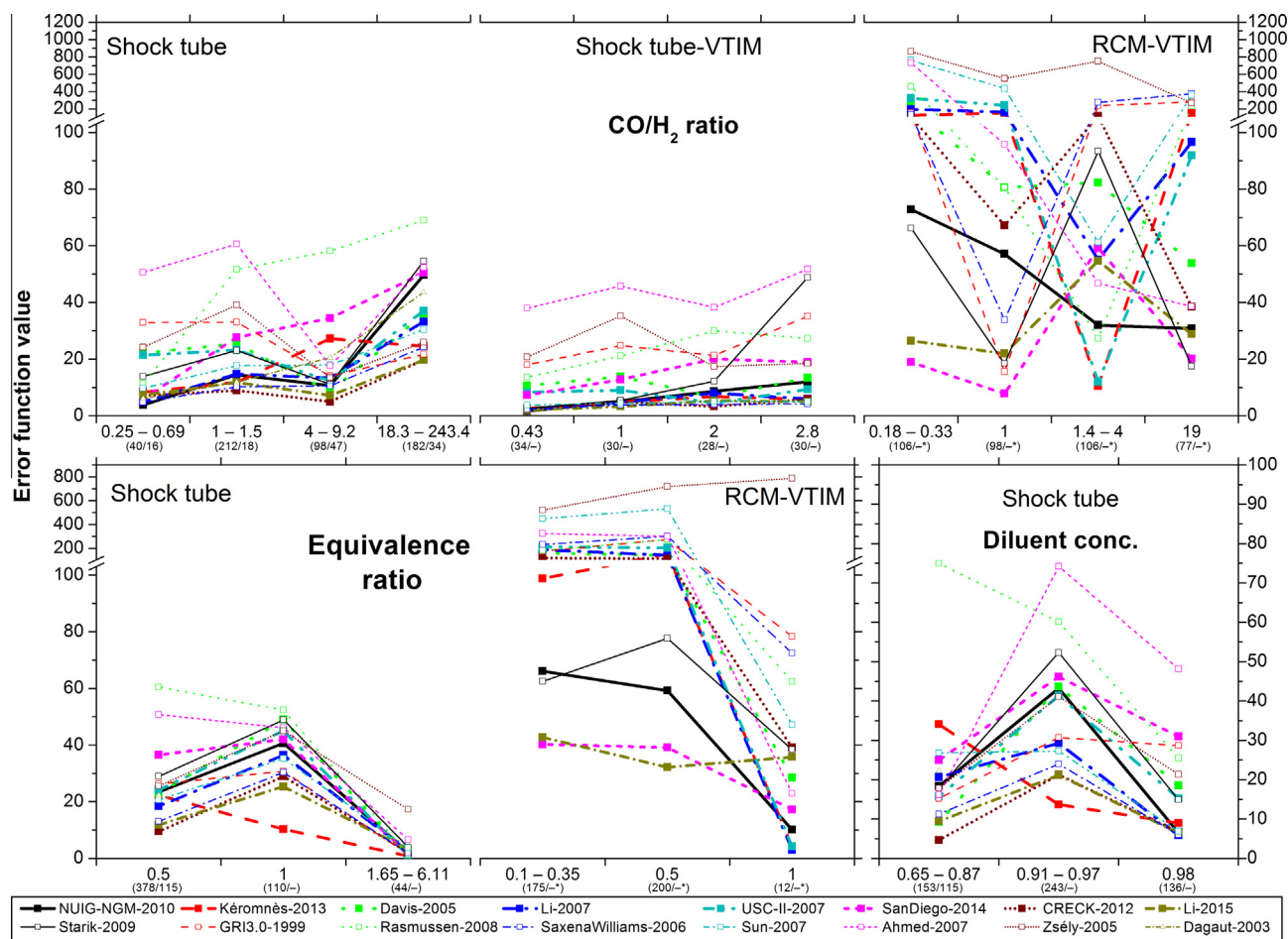
Fig. 4. Performance of the mechanisms for various ranges of \text{CO}/\text{H}_2 ratio, equivalence ratio and diluent concentration with respect to ignition delay time. Each plot shows the results for shock tubes (left part), shock tubes modeled using VTIM (middle part) and rapid compression machines (right part), if available. * – RCM results for Dagaut-2003 not shown (see text).
