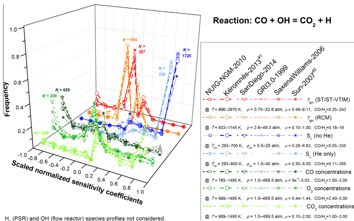
Fig. 14. Frequencies of sensitivity coefficients of reaction \text{CO} + \text{OH} = \text{CO}_2 + \text{H} for various types of measurements. The sensitivity analysis for this reaction was performed with the mechanisms NUIG-NGM-2010, Kéromnès-2013, SanDiego-2014, GRI3.0-1999, SaxenaWilliams-2006 and Sun-2007. The experimental conditions are given for each type of measurement.
