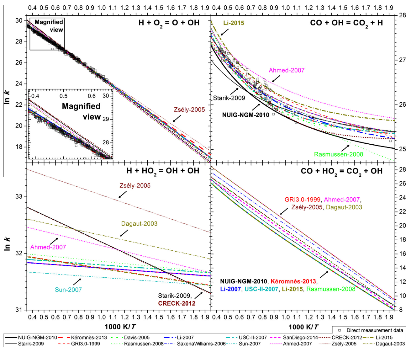
Fig. 12. Comparison of published reaction rate coefficients for the most sensitive reactions: \text{H} + \text{O}_2 = \text{O} + \text{OH} (top left panel), \text{CO} + \text{OH} = \text{CO}_2 + \text{H} (top right), \text{H} + \text{HO}_2 = \text{OH} + \text{OH} (bottom left) and \text{CO} + \text{HO}_2 = \text{CO}_2 + \text{OH} (bottom right). References to the direct measurements of reaction rate coefficients (black open squares) can be found in Table J of the Supplemental Material. The units of k are expressed in terms of cm, mol and s.
