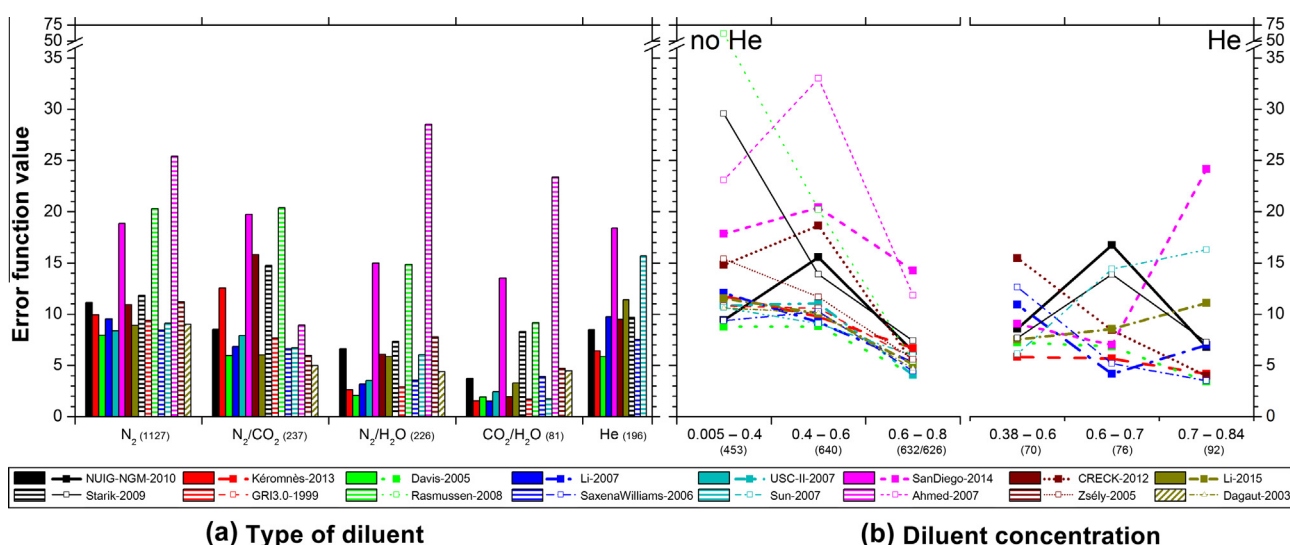
Fig. 5. (a) Error of the reproduction of the flame velocity according to the type of diluent system for the five most important diluent systems, (b) Performance of the mechanisms for various ranges of diluent concentration with respect to flame velocity for He-free (left part) and He-containing mixtures (right part).
