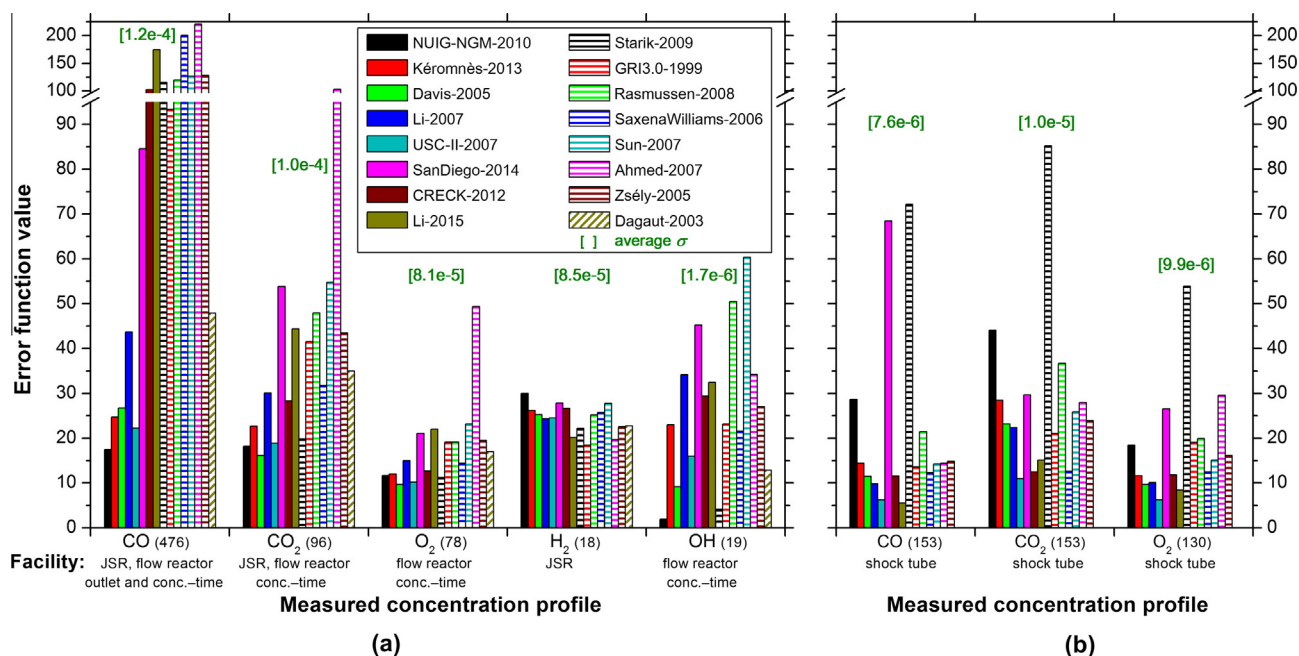
Fig. 7. Errors of the reproduction of concentration profiles depending on the measured profile for (a) JSR and flow reactor data and (b) shock tube data. The type of experimental methods in which the corresponding measurements were facilitated are given for each profile. Green numbers above the columns refer to average \sigma values for each subset.
