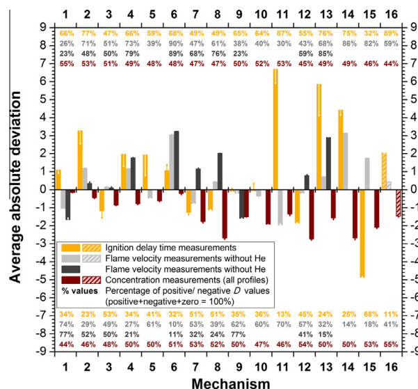
Fig. 11. Summary of average absolute deviation values of all mechanisms for ignition delay times, flame velocities and concentrations. The columns are striped if the number of data points differs from the other mechanisms (for Dagaut-2003, #16: all diluents except Ar and He). Identifying numbers were used for the mechanisms as in Table 1. Arrows indicate the changes of D values due the introduction of weighting as described in Section 6.4.
