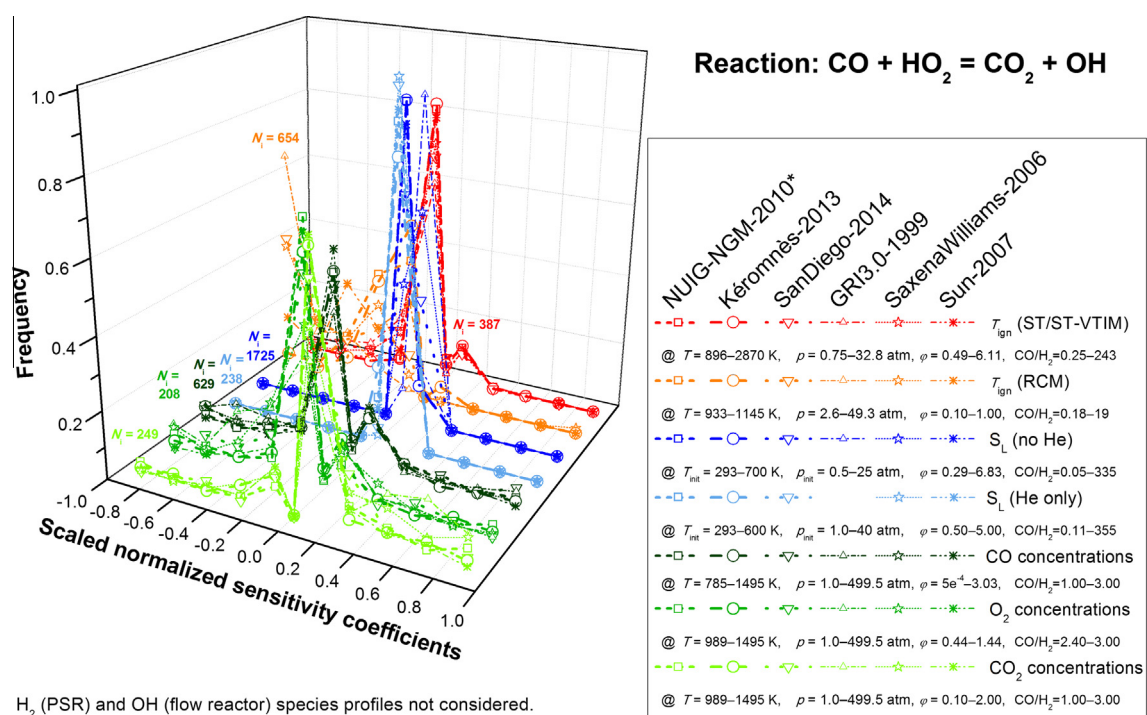
Fig. 16. Frequencies of sensitivity coefficients of reaction \text{CO} + \text{HO}_2 = \text{CO}_2 + \text{OH} for various types of measurements. The sensitivity analysis for this reaction was performed with the mechanisms NUIG-NGM-2010, Kéromnès-2013, SanDiego-2014, GRI3.0-1999, SaxenaWilliams-2006 and Sun-2007. The experimental conditions are given for each type of measurement.
