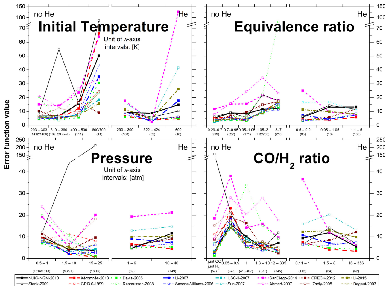
Fig. 6. Performance of the mechanisms for various ranges of temperature, equivalence ratio, pressure and CO/H 2 ratio with respect to flame velocities. Each plot shows the results for He-free mixtures (left part) and He-containing mixtures (right part). Note that those mechanisms without He as a defined species do not appear in the right part of the plots.
