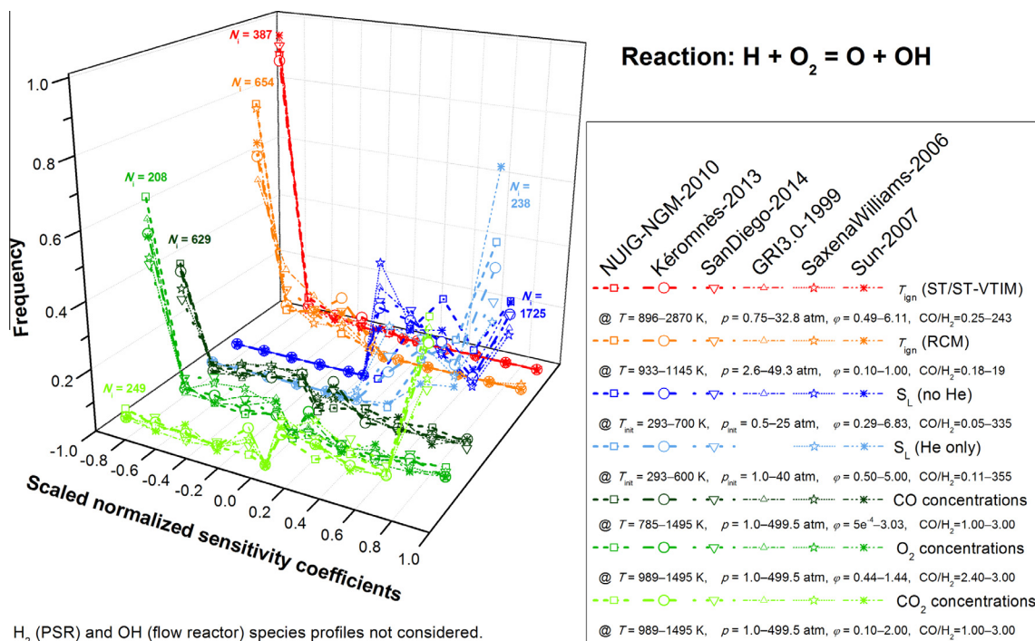
Fig. 13. Frequencies of sensitivity coefficients of reaction \text{H} + \text{O}_2 = \text{O} + \text{OH} for various types of measurements. The sensitivity analysis for this reaction was performed with the mechanisms NUIG-NGM-2010, Kéromnès-2013, SanDiego-2014, GRI3.0-1999, SaxenaWilliams-2006 and Sun-2007. The experimental conditions are given for each type of measurement.
