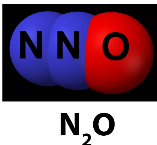
Figure 6.11: Chemical structure of dinitrogen oxide (nitrous oxide).
