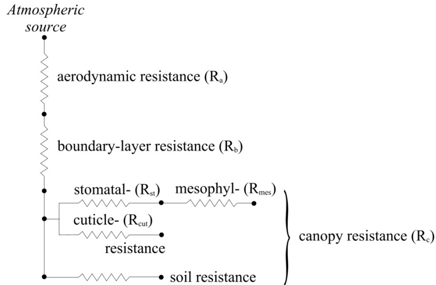
Figure 12.3: A widely used simple resistance network in dry deposition models
