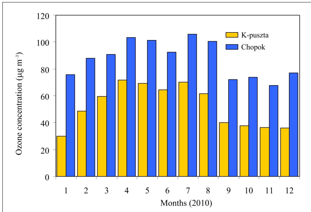
Figure 8.10: Average monthly ozone concentrations in 2010 at two EMEP (European Monitoring and Evaluation Programme) measuring station: K-puszta (Hungary, \phi = 46^{\circ}58' , \lambda = 19^{\circ}35' , h = 125 m) and Chopok (Slovakia, \phi = 48^{\circ}56' , \lambda = 19^{\circ}35' , h = 2008 m). Source of data: http://www.nilu.no/projects/ccc/onlinedata/
