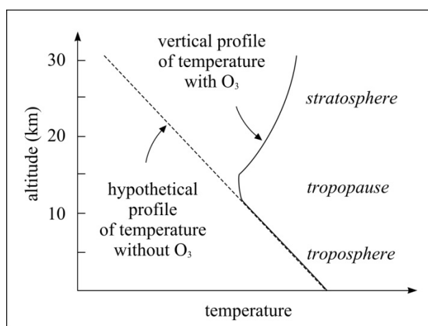
Figure 1.10: Real and hypothetical vertical profile of temperature with and without ozone in the stratosphere, respectively.
