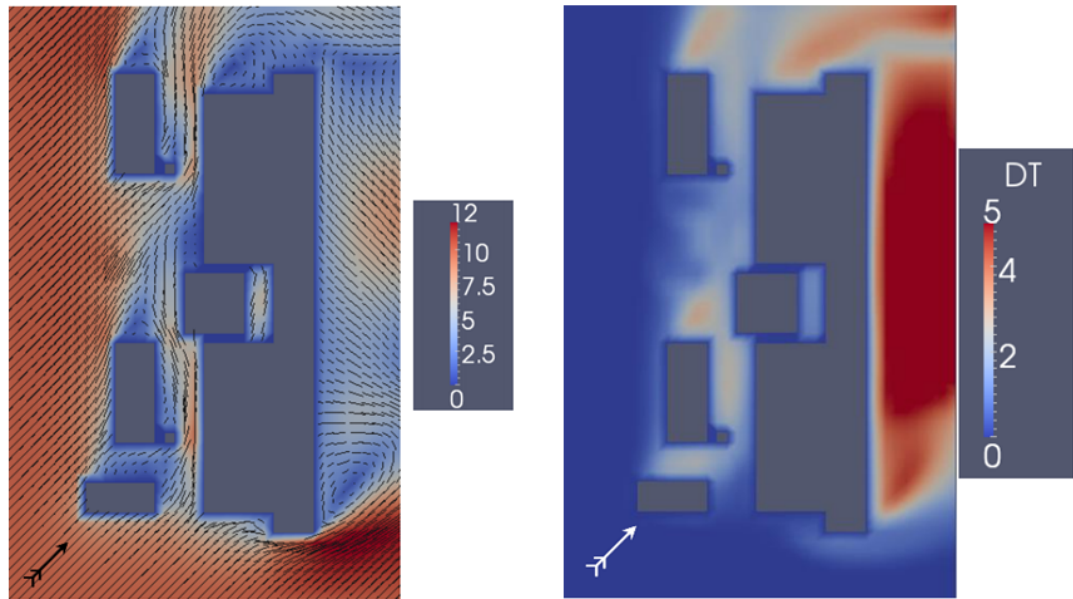
Figure 10.9: Horizontal cross section of the wind field (m/s) and turbulent diffusion coefficient ( \text{m}^2/\text{s} ) at 10 m height around the buildings of the Paks Nuclear Power Plant, assuming 10 m/s south-westerly wind. On the lee side, turbulent diffusion dominates over advection.
