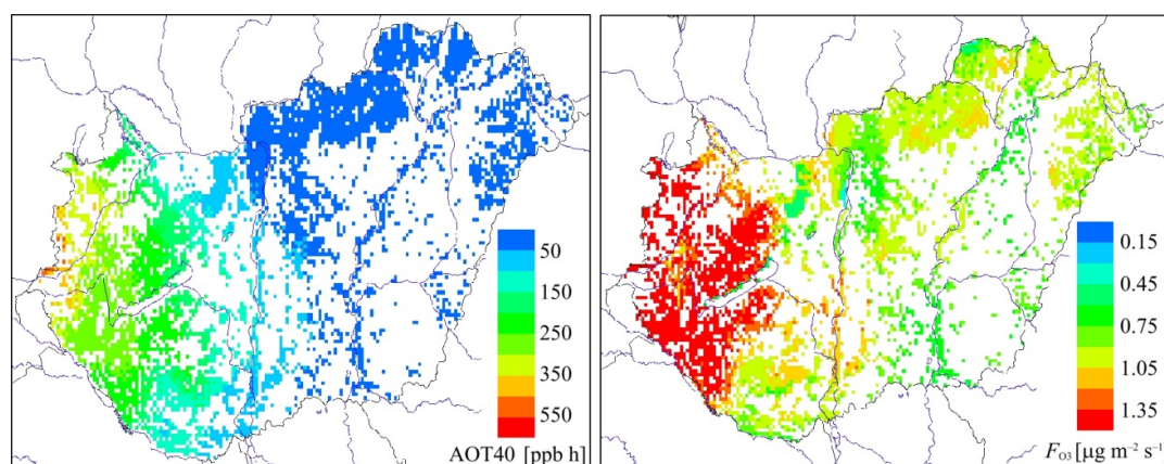
Figure 13.10: Estimated AOT40 and total flux of ozone over deciduous forest in Hungary in July 1998. Model simulations were carried out by TREX transport-deposition model (Eötvös Loránd University). Meteorological data were obtained from ALADIN numerical weather prediction model used at Hungarian Meteorological Service.
