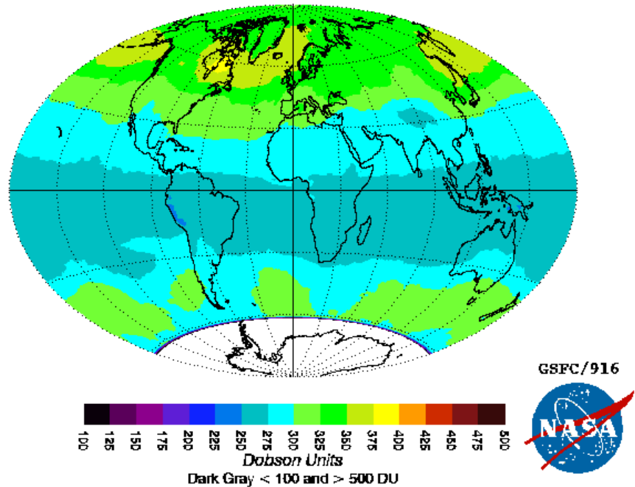
Figure 15.10: Average total vertical ozone concentration of June 2000, measured by space-based UV-spectrophotometer (source: NASA)
