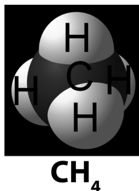
Figure 5.4: Chemical structure of methane.
