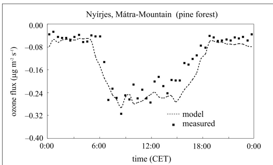
Figure 12.5. Average daily courses of measured and modelled dry deposition flux of ozone ( O_3 ). Results are obtained from eddy covariance measurements over pine forest (Nyírjes, Hungary) and model simulations.
