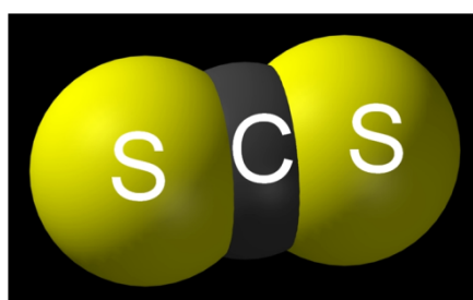
Figure 7.4: Chemical structure of sulphur compounds – carbonyl sulphide (Source: Wikipedia).
