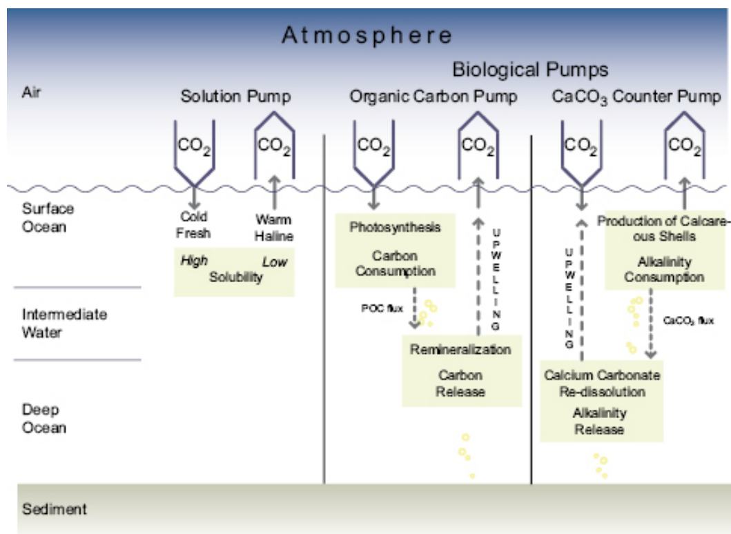
Figure 5.6: Physical pump and biological pump. Three main ocean carbon pumps govern the regulation of natural atmospheric CO 2 changes by the ocean (Heinze et al., 1991): the solubility pump, the organic carbon pump and the CaCO 3 ‘counter pump’. The oceanic uptake of anthropogenic CO 2 is dominated by inorganic carbon uptake at the ocean surface and physical transport of anthropogenic carbon from the surface to deeper layers. For a constant ocean circulation, to first order, the biological carbon pumps remain unaffected because nutrient cycling does not change. If the ocean circulation slows down, anthropogenic carbon uptake is dominated by inorganic buffering and physical transport as before, but the marine particle flux can reach greater depths if its sinking speed does not change, leading to a biologically induced negative feedback that is expected to be smaller than the positive feedback associated with a slower physical downward mixing of anthropogenic carbon. Source IPCC AR4 Fig. 7.10
