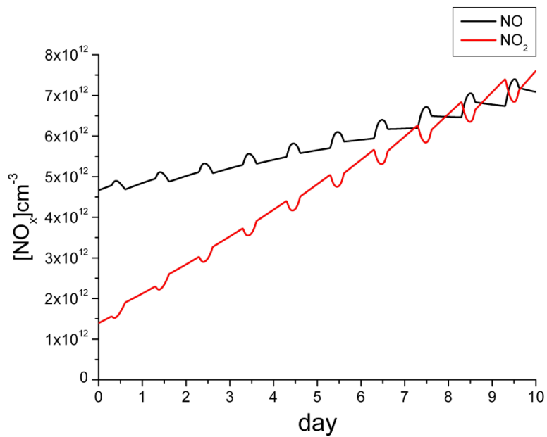
Figure 3.9: Results of the numerical simulations using CBM Leeds mechanism – variation of \text{NO}_x in winter time.
