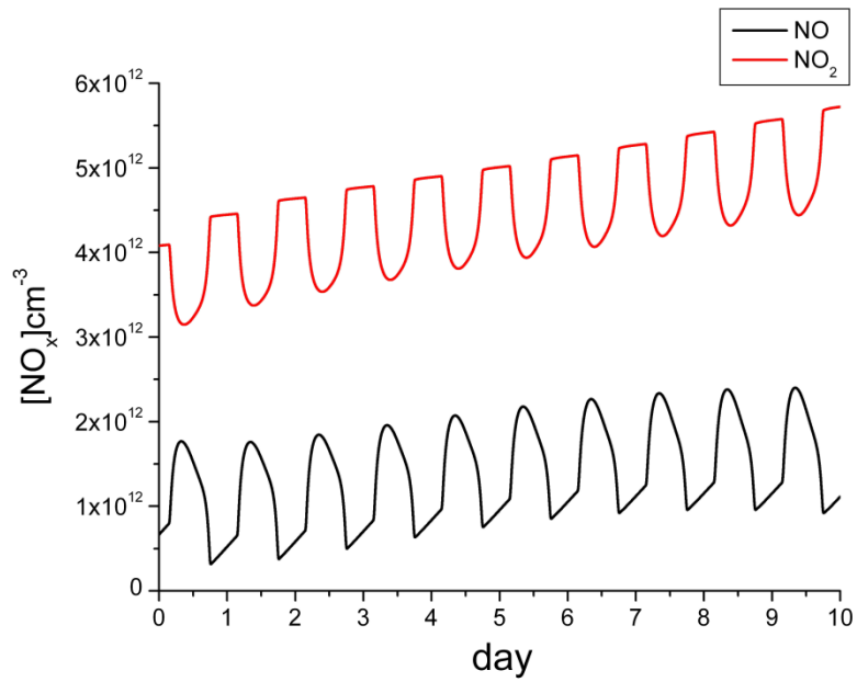
Figure 3.8: Results of the numerical simulations using CBM Leeds mechanism – variation of \text{NO}_x in summer time.
