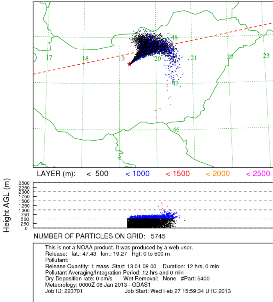
Figure 10.6: Dispersion of particles in the HYSPLIT model.
