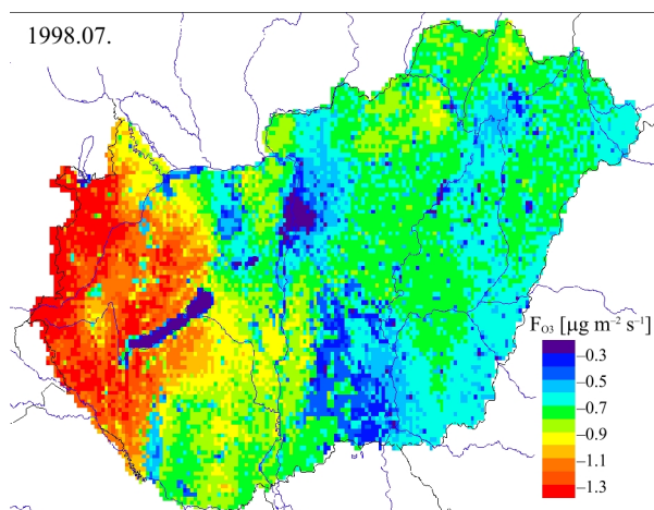
Figure 12.10: Average daytime deposition flux of the ozone ( O_3 ) in July 1998 over Hungary. Results are obtained from model simulations. (Negative sign denotes that the flux is downward.)
