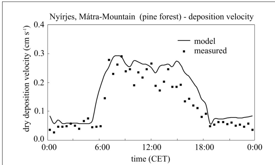
Figure 12.6: Average daily courses of measured and modelled dry deposition velocity of ozone ( O_3 ). Results are obtained from eddy covariance measurements over pine forest (Nyírjes, Hungary) and model simulations.
