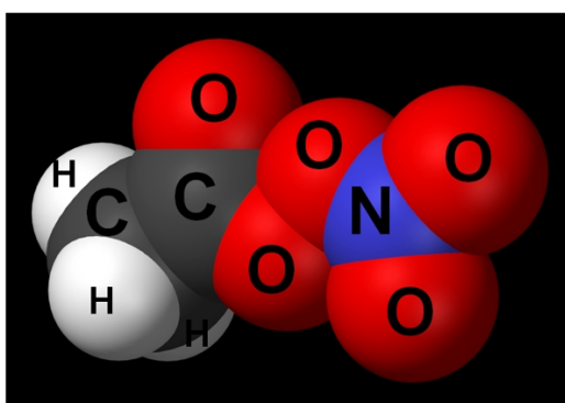
Figure 6.8: Chemical structure of nitric acid.
