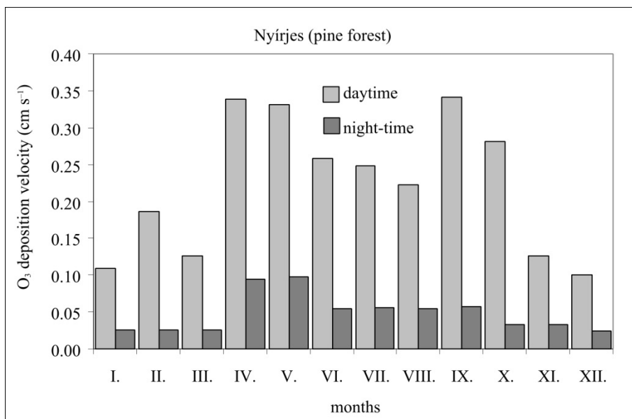
Figure 12.7: Monthly averages of daytime and night-time deposition velocity for ozone ( O_3 ) in 1998 over pine forest (Nyírjes, Mátra Mountain). Results are obtained from model simulations.
