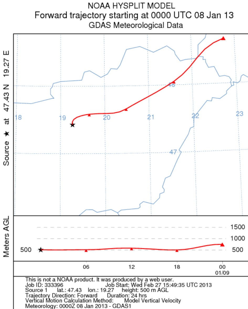
Figure 10.5: Air mass (or single particle) trajectory in the HYSPLIT model.
