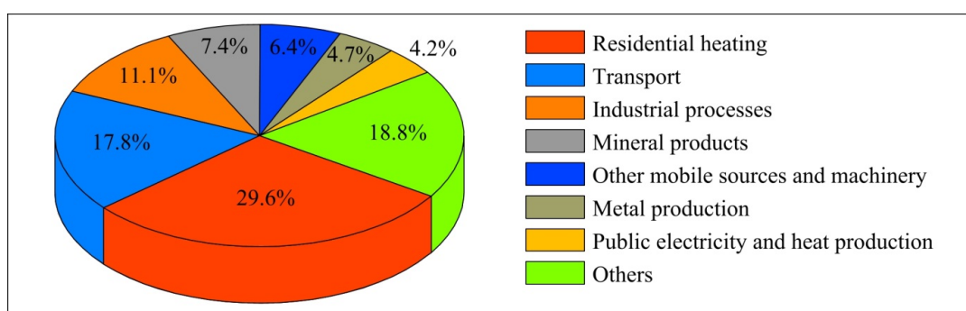
Figure 2.15: Emission sources of particulate matter, PM2.5 in 2006 in EU27. Emission data are calculated by the estimations of member countries.
