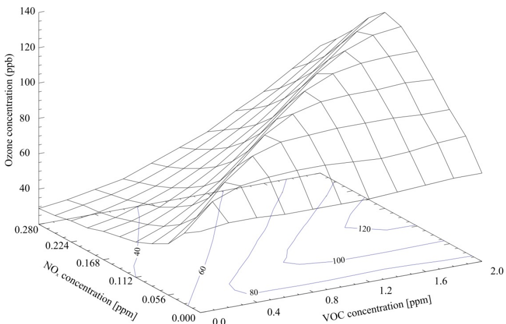
Figure 8.11: Modelled ozone concentration with different ratio of NO x and VOC concentration
