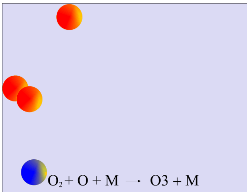
Figure 8.2: Production of ozone from an oxygen atom and an oxygen molecule in the presence of a third molecule (usually N_2 , or another O_2 ).
